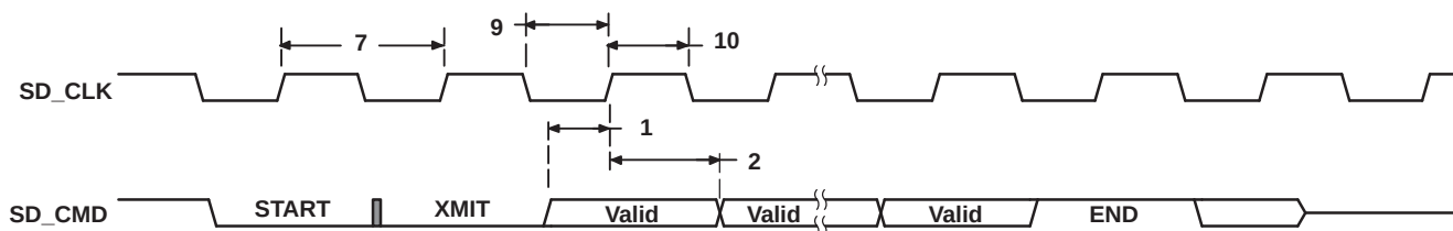
Figure 5-41. MMC/SD Card Response Timing
