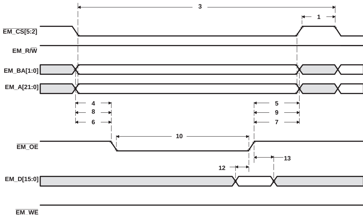
Figure 5-19. Asynchronous Memory Read Timing for EMIF
