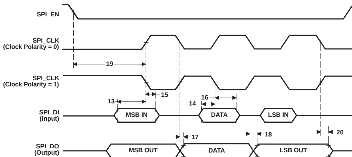
Figure 5-59. SPI Master Mode External Timing (Clock Phase = 1)
