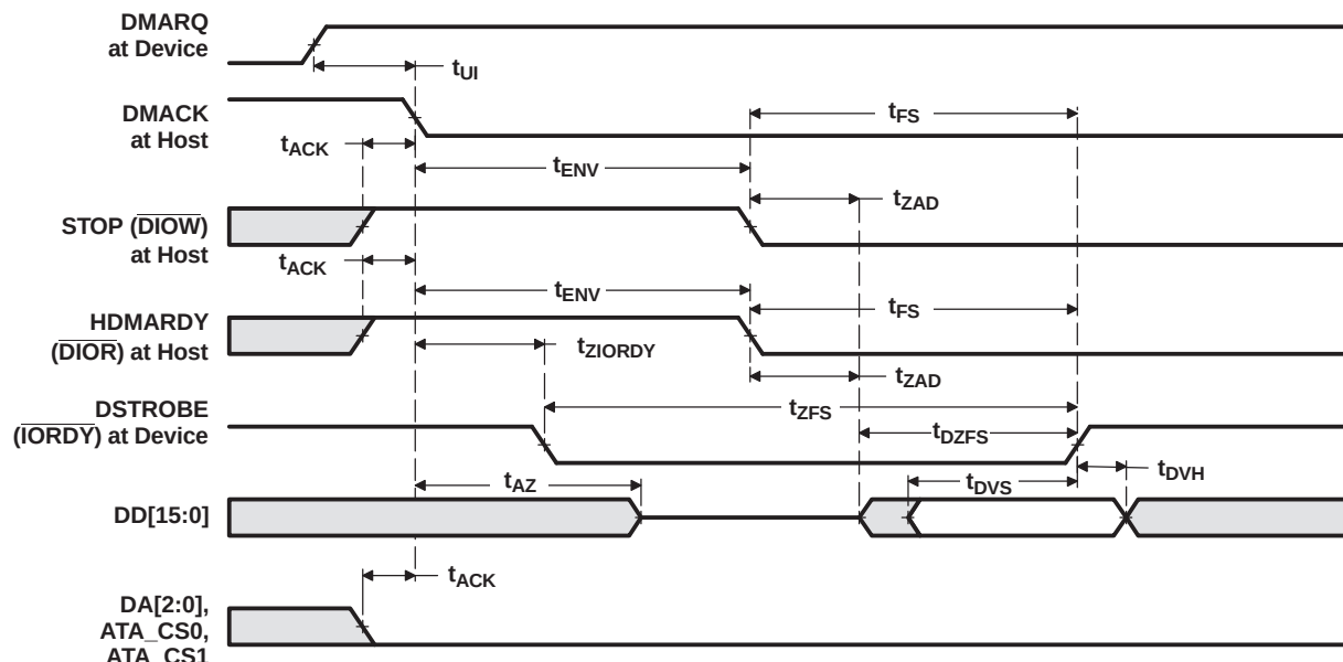
Figure 5-26. ATA/CF Initiating an Ultra DMA Data-In Burst Timing
