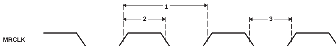
Figure 5-64. MRCLK Timing (EMAC - Receive)
