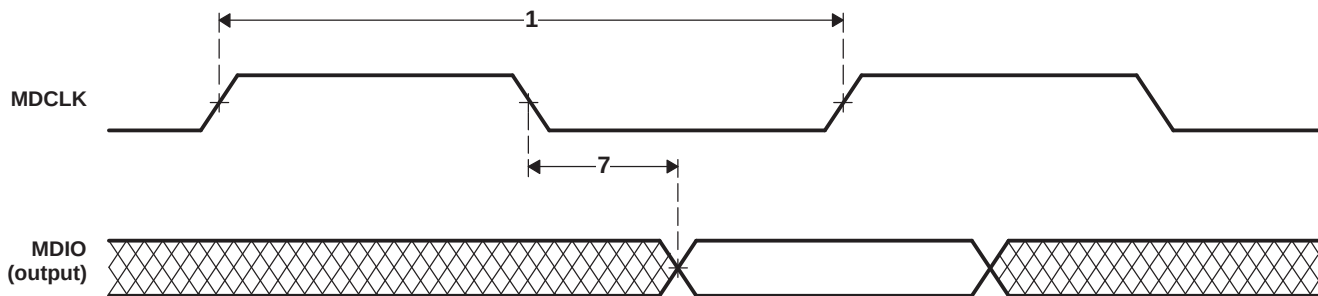
Figure 5-69. MDIO Output Timing
