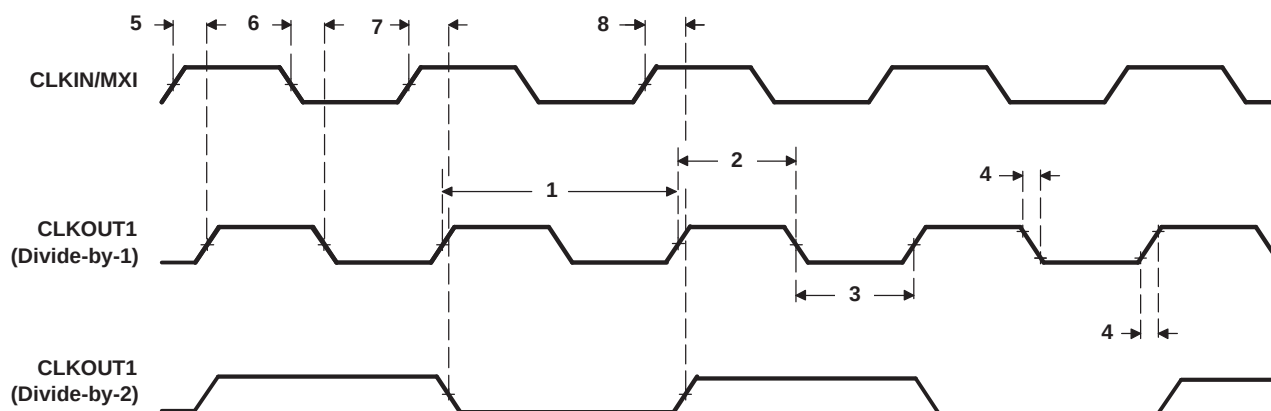
Figure 5-15. CLKOUT1 Timing
