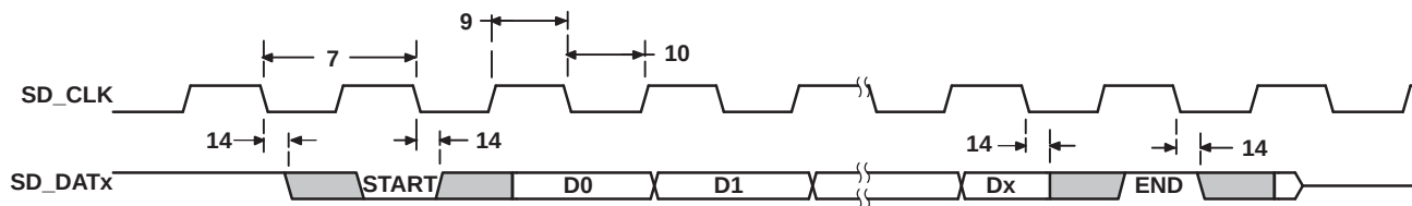
Figure 5-42. MMC/SD Host Write Timing
