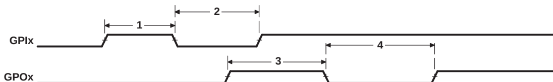
Figure 5-17. GPIO Port Timing
