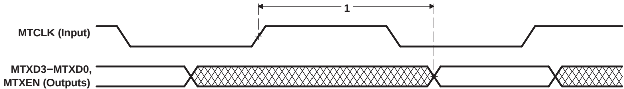
Figure 5-67. EMAC Transmit Interface Timing
