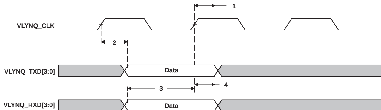
Figure 5-74. VLYNQ Transmit/Receive Timing
