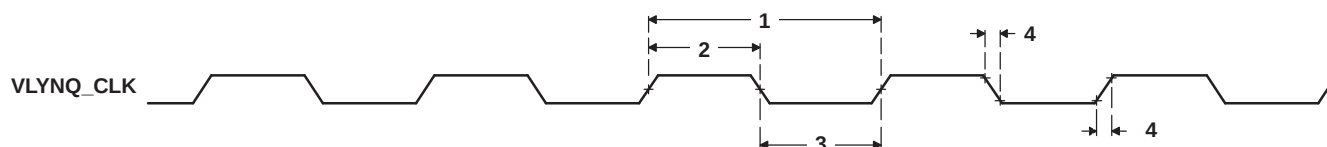
Figure 5-73. VLYNQ_CLK Timing for VLYNQ
