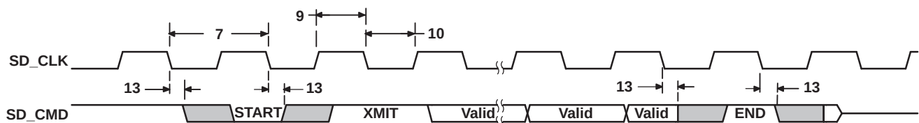
Figure 5-40. MMC/SD Host Command Timing
