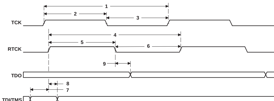
Figure 5-76. JTAG Test-Port Timing
