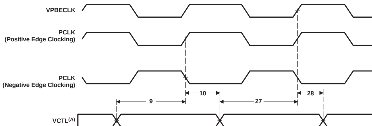
Figure 5-49. VPBE Input Timing With Respect to PCLK and VPBECLK
