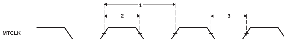
Figure 5-65. MTCLK Timing (EMAC - Transmit)
