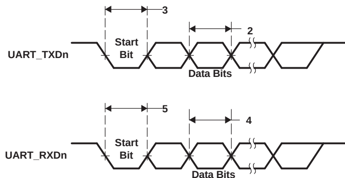
Figure 5-56. UART Transmit/Receive Timing
