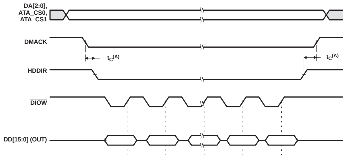
Figure 5-38. ATA/CF HDDIR Multiword DMA Write Transfer Timing
