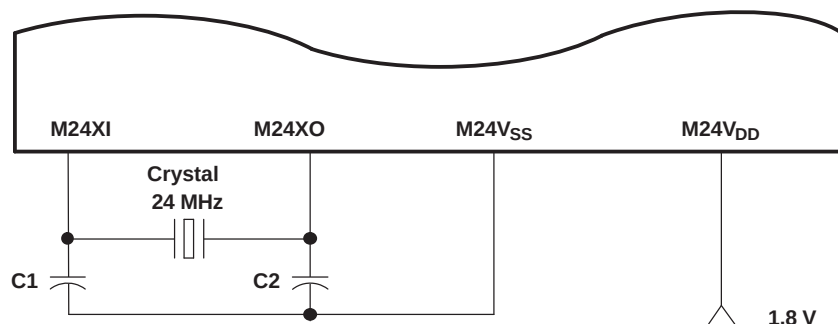
Figure 5-11. 24-MHz USB Oscillator
