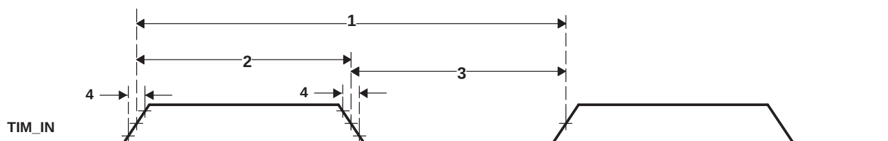
Figure 5-70. Timer Timing
