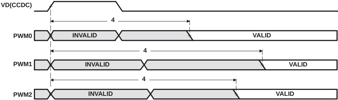
Figure 5-72. PWM Output Delay Timing
