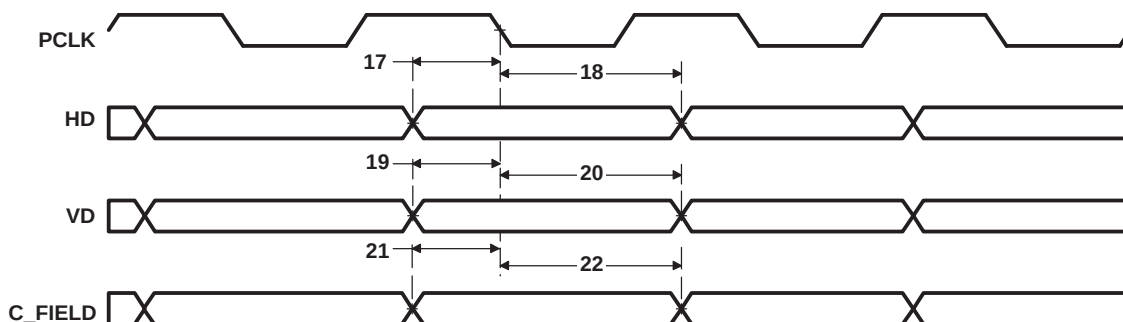
Figure 5-47. VPFE (CCD) Master Mode Control Output Data Timing
