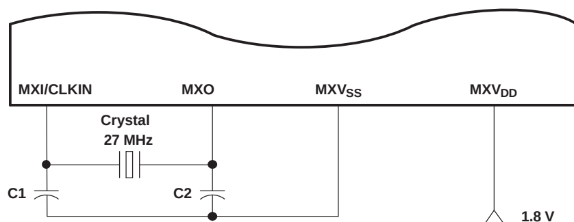
Figure 5-10. 27-MHz System Oscillator
