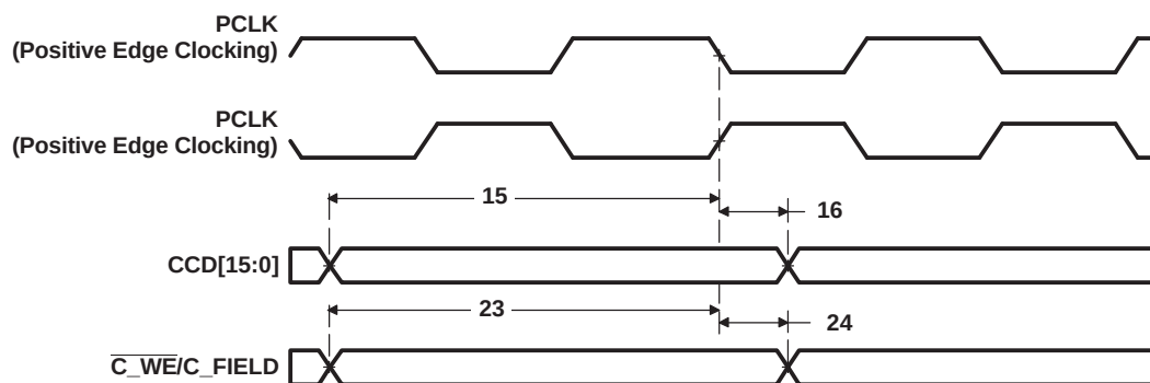
Figure 5-46. VPFE (CCD) Master Mode Input Data Timing
