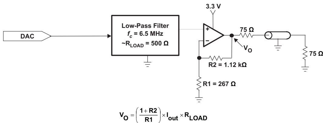
Figure 5-53. Typical Output Circuit for NTSC/PAL Video From DACs
