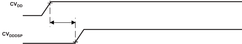
Figure 5-4. DSP Host-Boot Mode Core Supply Timings
