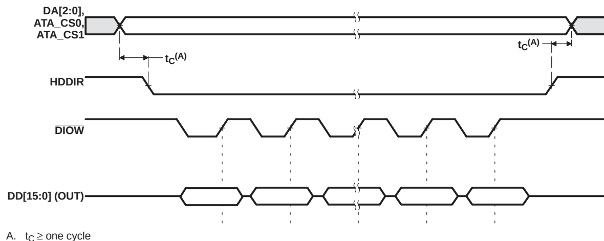
Figure 5-37. ATA/CF HDDIR PIO Postwrite Start Timing
