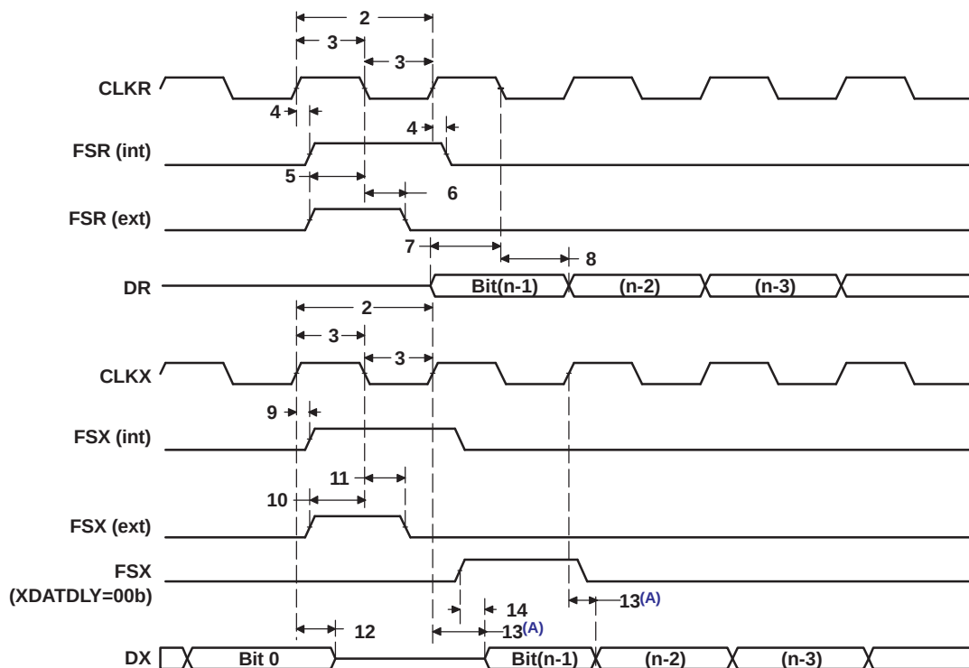
Figure 5-63. ASP Timing
