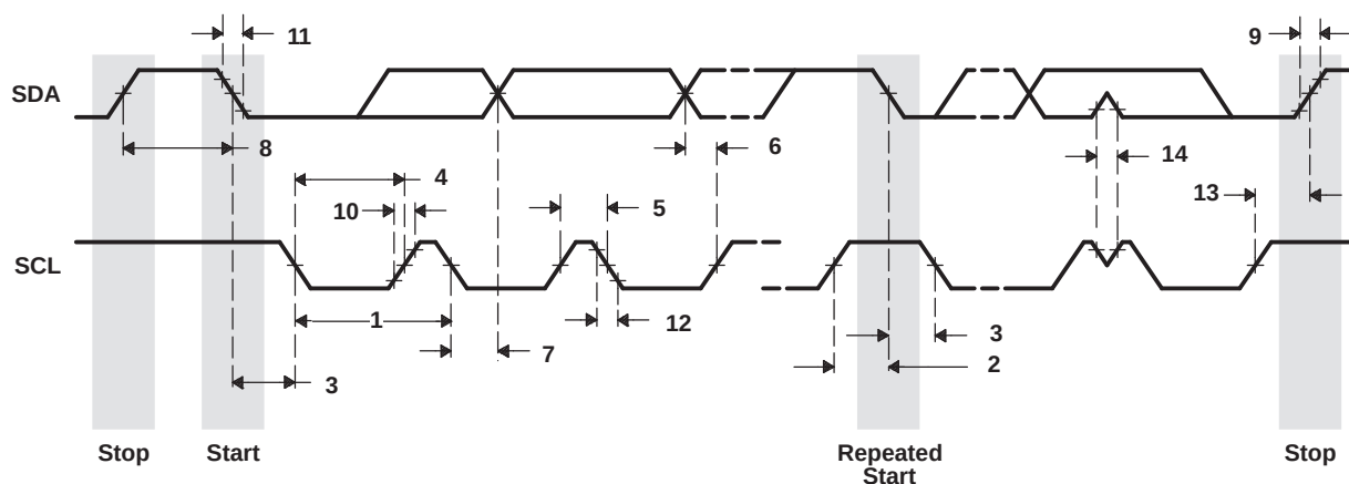
Figure 5-61. I2C Receive Timings
