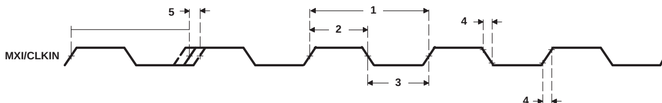
Figure 5-12. MXI/CLKIN Timing
