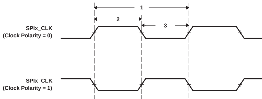
Figure 5-57. SPI_CLK Timing
