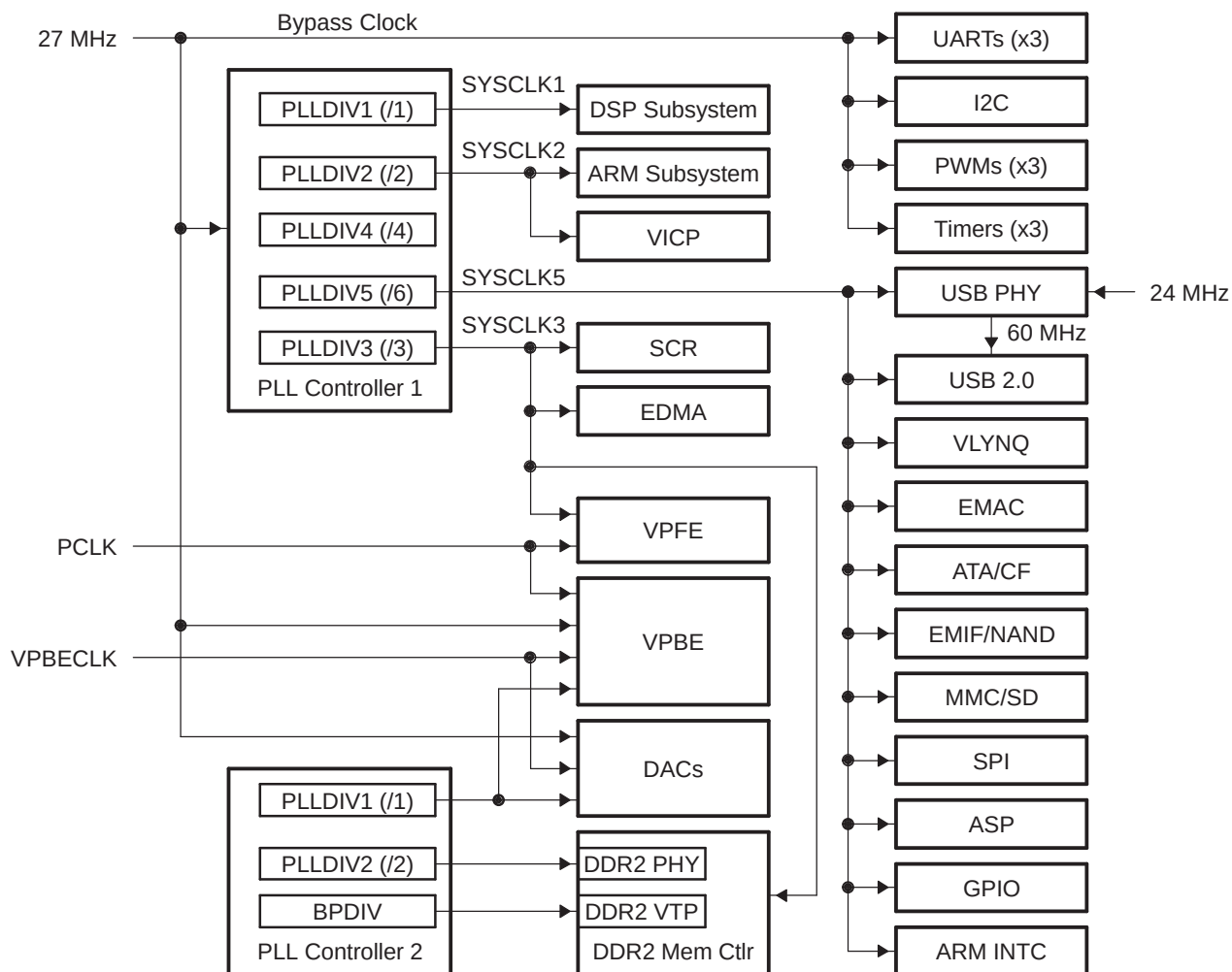
Figure 5-6. PLL1 and PLL2 Clock Domain Block Diagram
