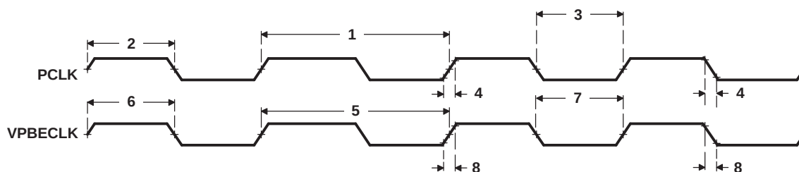
Figure 5-48. VPBE PCLK and VPBECLK Timing
