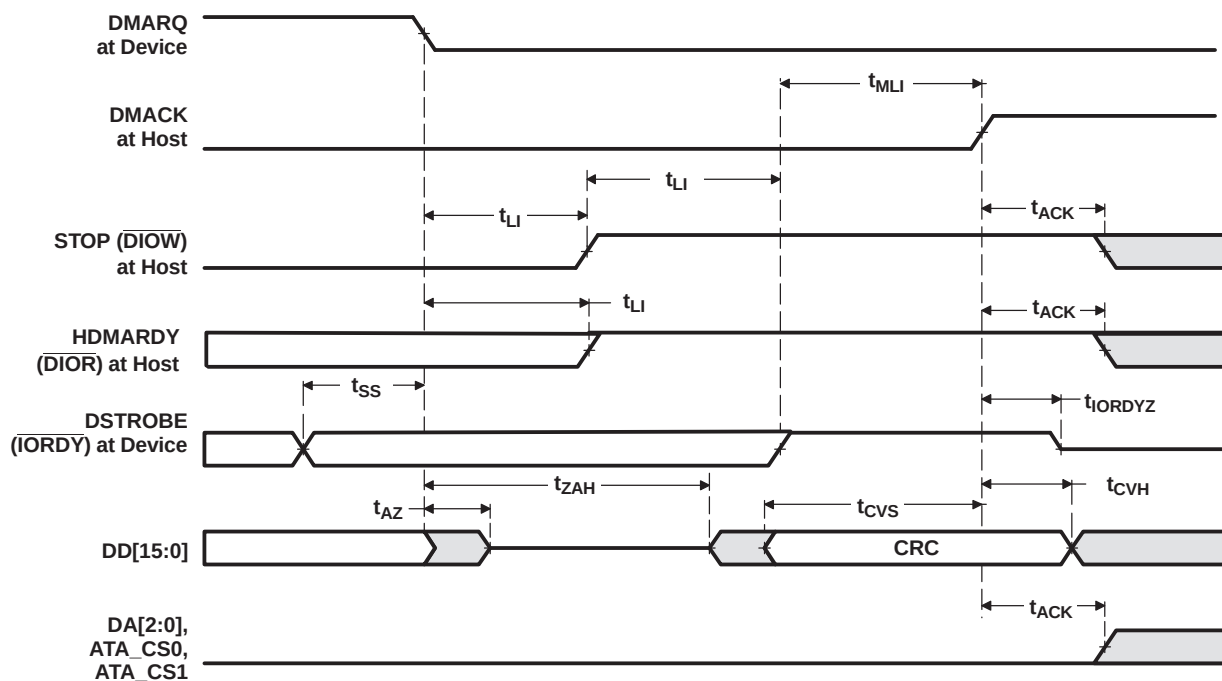
Figure 5-29. ATA/CF Device Terminating an Ultra DMA Data-In Burst Timing
