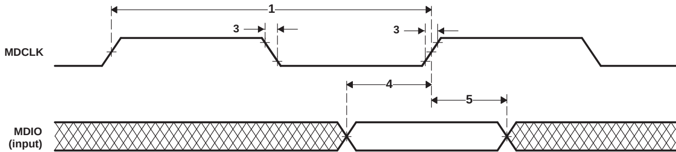
Figure 5-68. MDIO Input Timing
