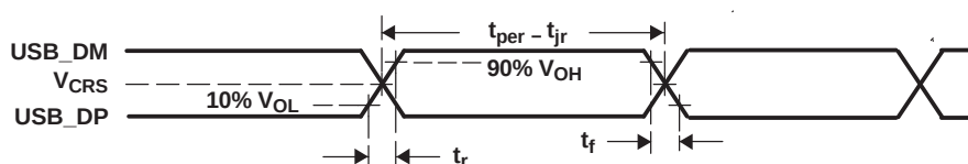
Figure 5-55. USB2.0 Integrated Transceiver Interface Timing
