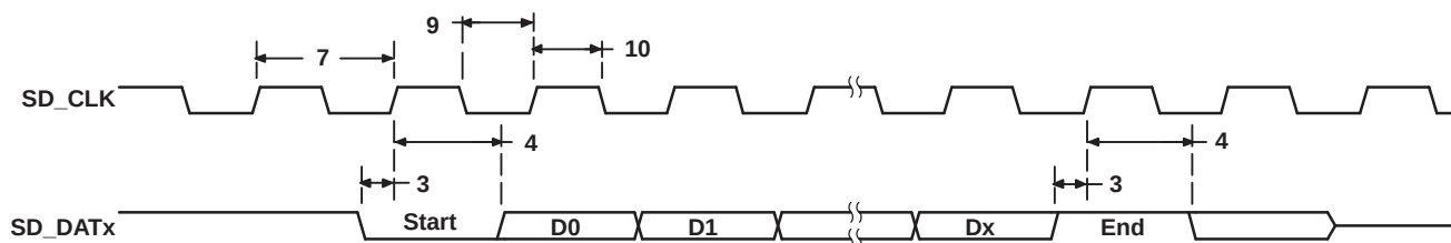
Figure 5-43. MMC/SD Host Read and Card CRC Status Timing
