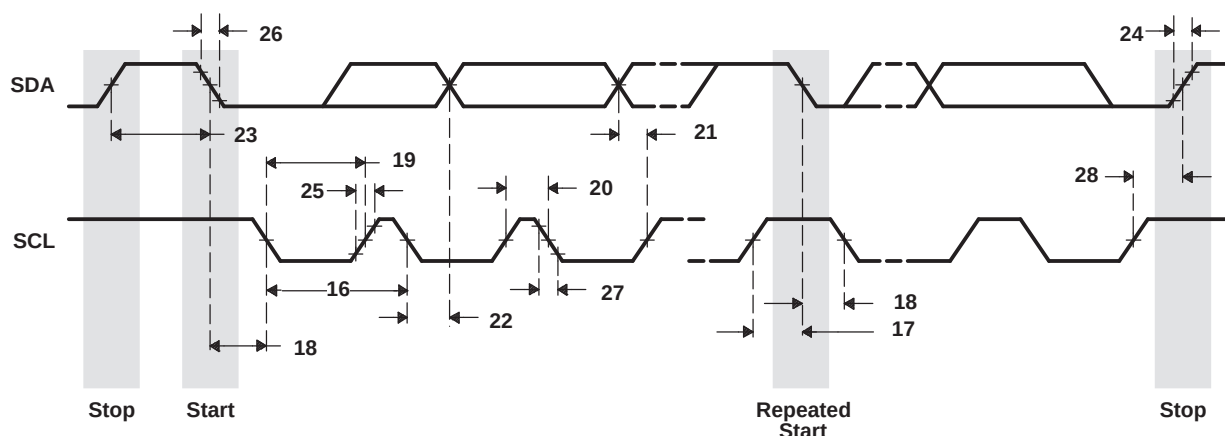
Figure 5-62. I2C Transmit Timings
