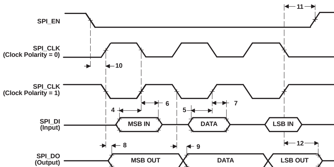
Figure 5-58. SPI Master Mode External Timing (Clock Phase = 0)
