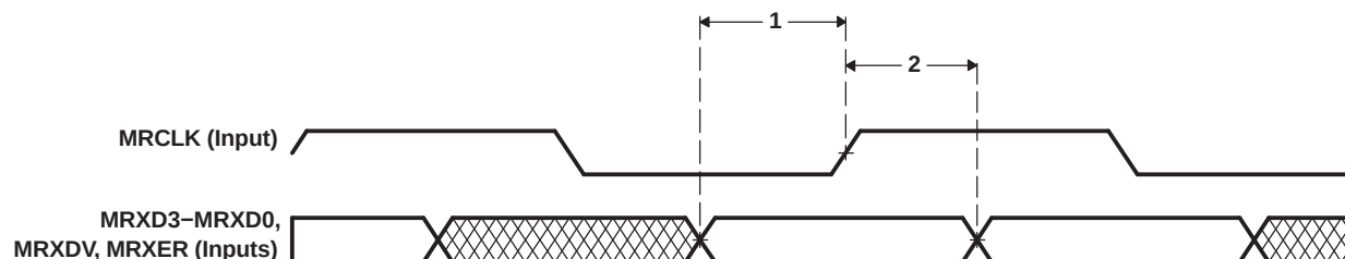
Figure 5-66. EMAC Receive Interface Timing
