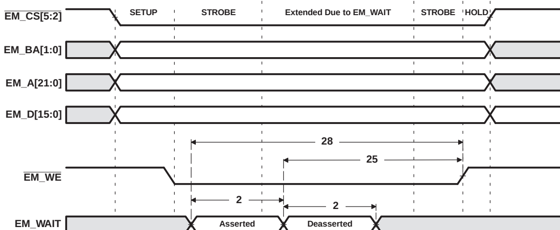
Figure 5-22. EM_WAIT Write Timing Requirements
