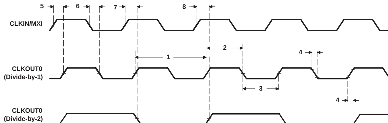
Figure 5-14. CLKOUT0 Timing
