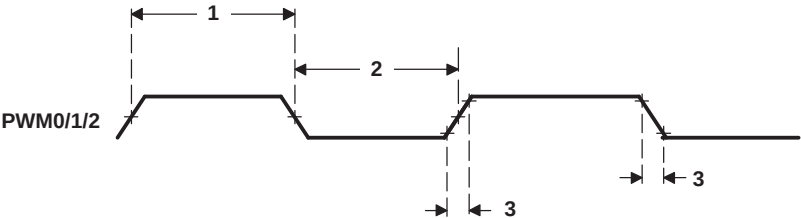
Figure 5-71. PWM Output Timing
