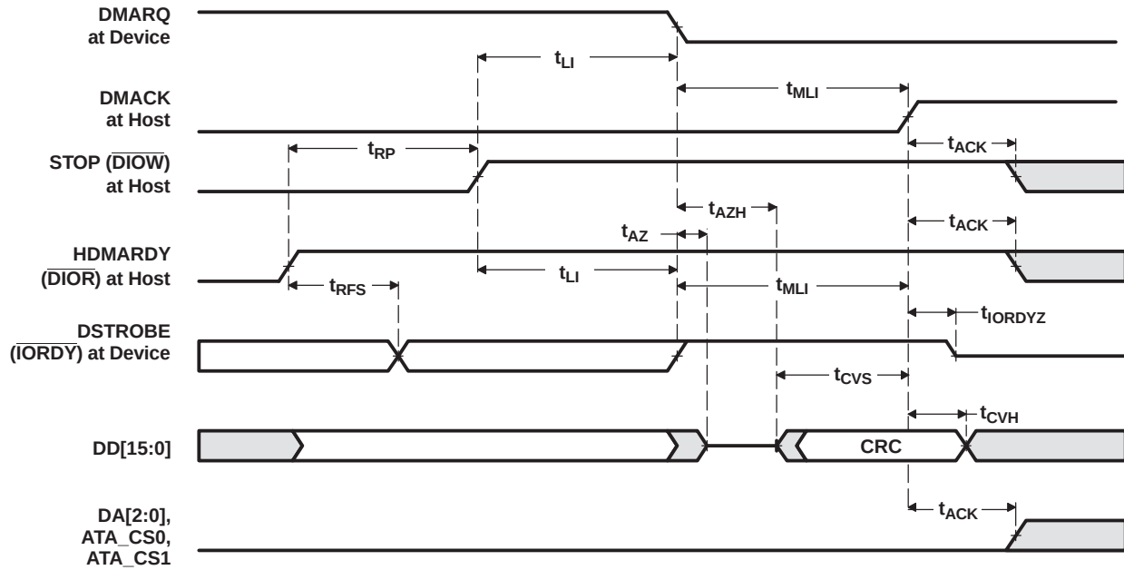
Figure 5-30. ATA/CF Host Terminating an Ultra DMA Data-In Burst Timing
